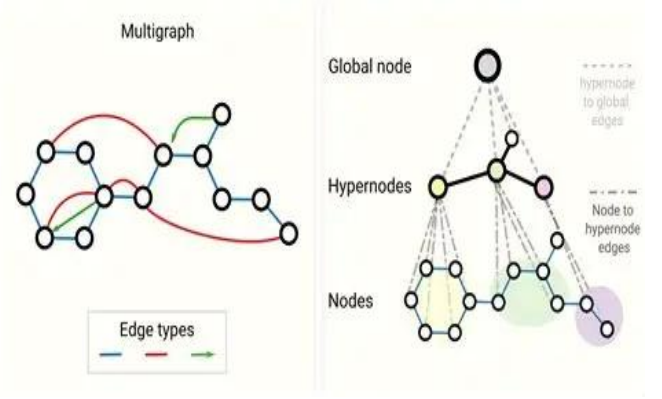
Fig. 2. Graph Neural Networks architecture
